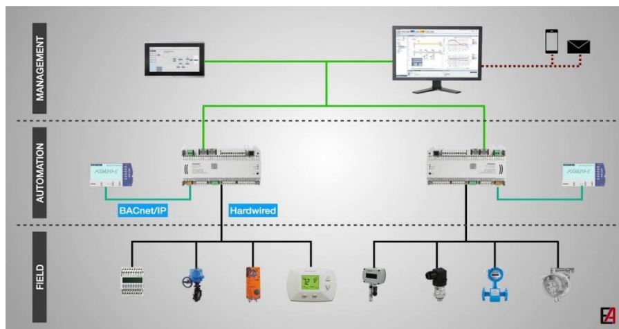
Fig:- BMS System
